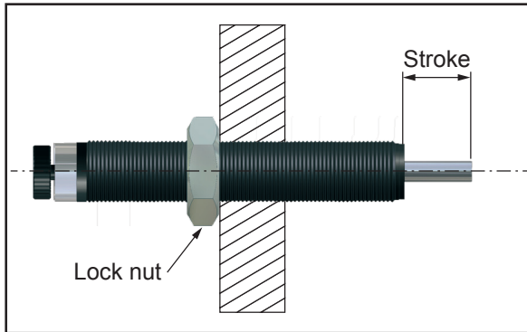
Installation with Lock nut
