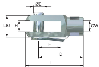
3 Female rod clevis (DIN 71752)
