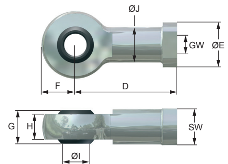
4 Spherical end bearing (DIN 648, Series K)
