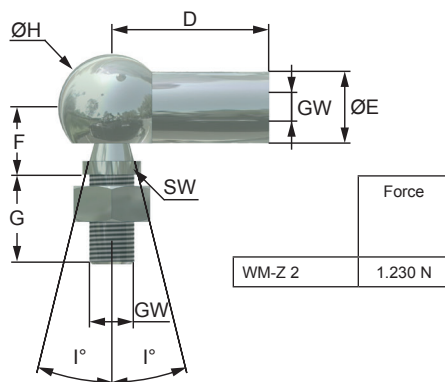
2 Angle joint (DIN 71802)
